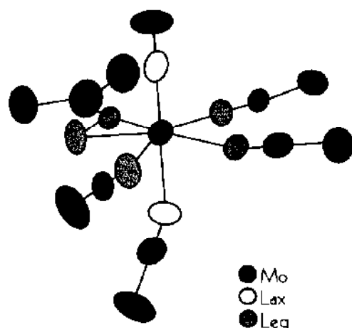
Fig. 2. Molecular structure of [\text{Mo}(\text{NO})(\text{OCN}(\text{CH}_3)_2)(\text{NCS})_4]^{2-} (without H-atoms) [30].
